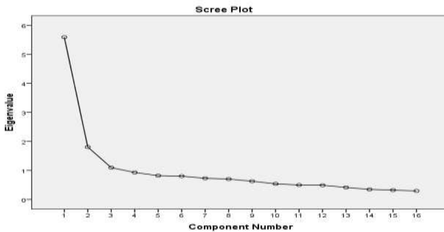
Figure 1. Scree plot
